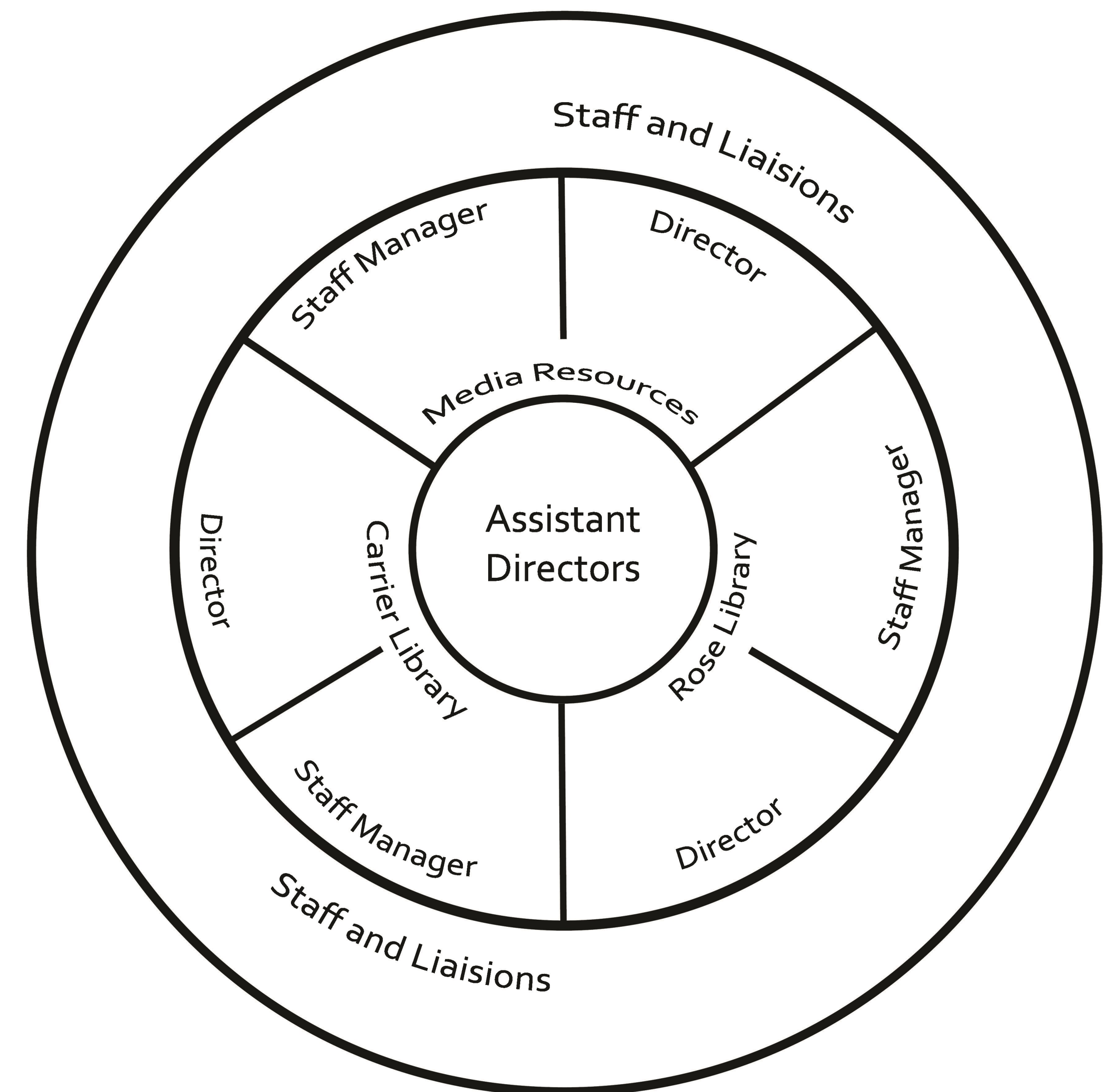
Collaborative Model
